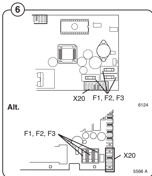
Fig. 6 2. Verify that the voltage supply to the programme is as shown in the table below. Measure on card terminal X20.
