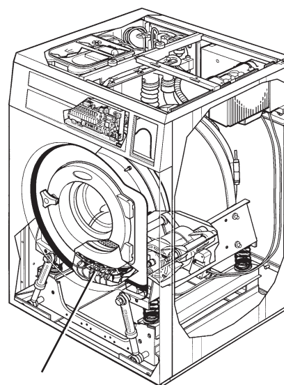
Element connectors
